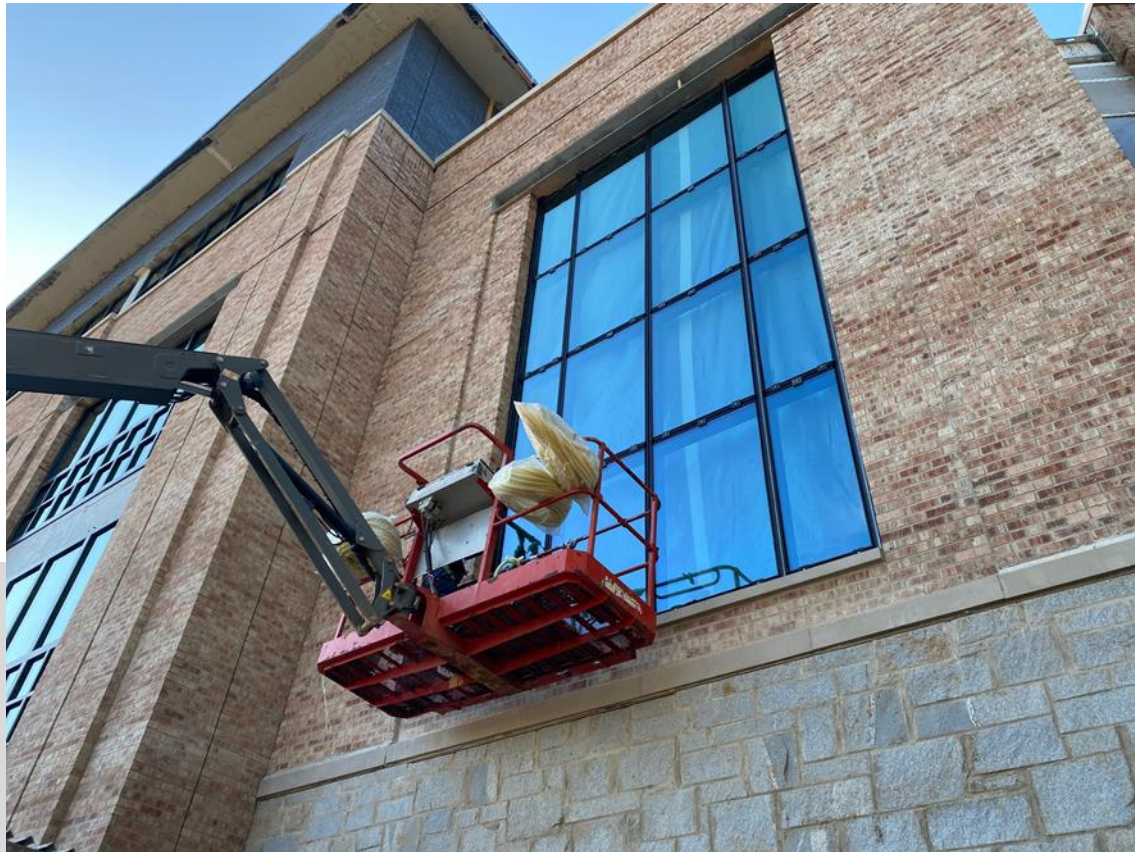
Curtainwall Install at North West Elevation
